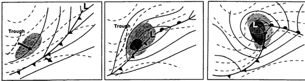
Fig. 1: Scheme of cyclogenesis due to approach and superposition of an upper vorticity maximum ( embedded in a trough) on a slower moving frontal zone in lower levels. Shading represents the region of appreciable positive vorticity advection (PVA) aloft. From Petterssen (1956).
