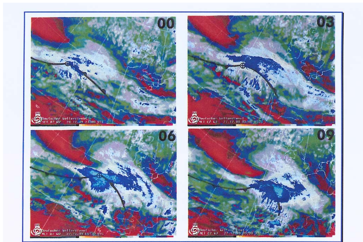
Fig.4: WV-images of METEOSAT from 27-12-99, 00, 03, 06 and 09 UTC with surface fronts and position of the surface low.
